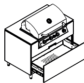
120 Slide-in grill 1200 x 770 x 915mm 48" x 30" x 36"
