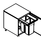
60 Pull-out bin 600 x 770 x 915mm 24" x 30" x 36"
