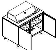
120 Drop-in grill 1200 x 770 x 915mm 48" x 30" x 36"
